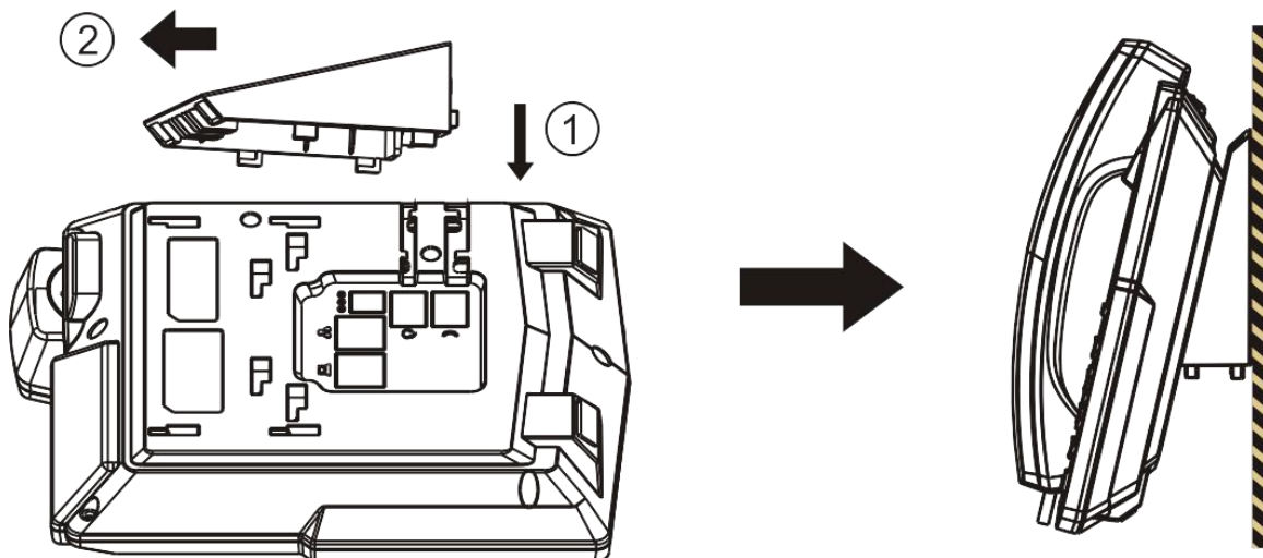
Figure 2 - Wall-mount Installation
